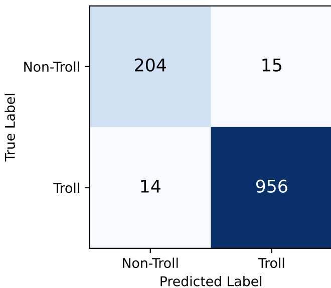
(c) Classification-only Baseline
