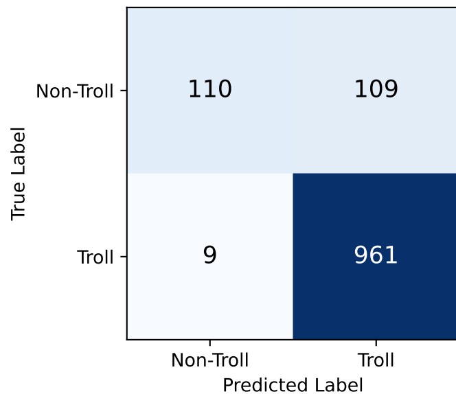
(b) TF-IDF + SGD
