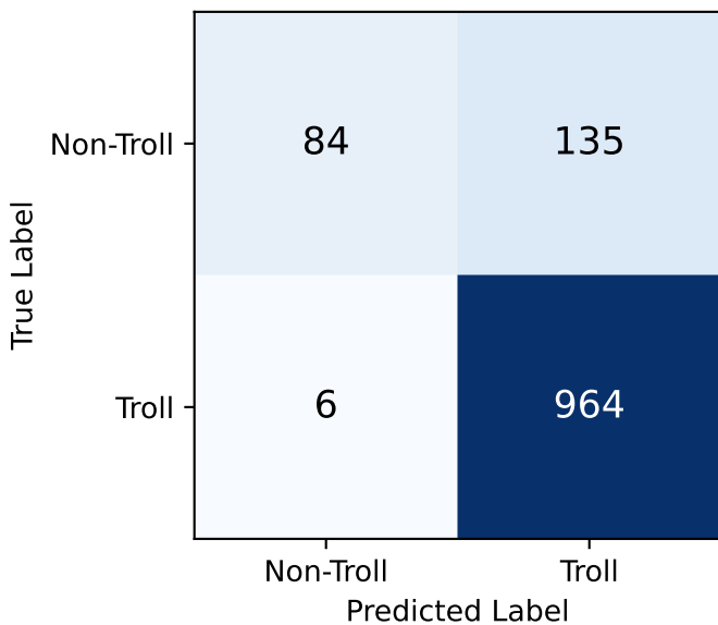
(a) TF-IDF + Logistic Regression
